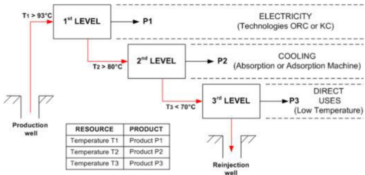
Figure 3: Cascade use geothermal energy combining various technologies, with ORC : stand-alone, flexible and portable production modules for in the range of 20 to 200 kWe, a size adapted to the production expected, coupled with cascade direct uses of the fluid serving other local needs at the low temperature, ending with the use of the water itself (Varet et al., 2014).
