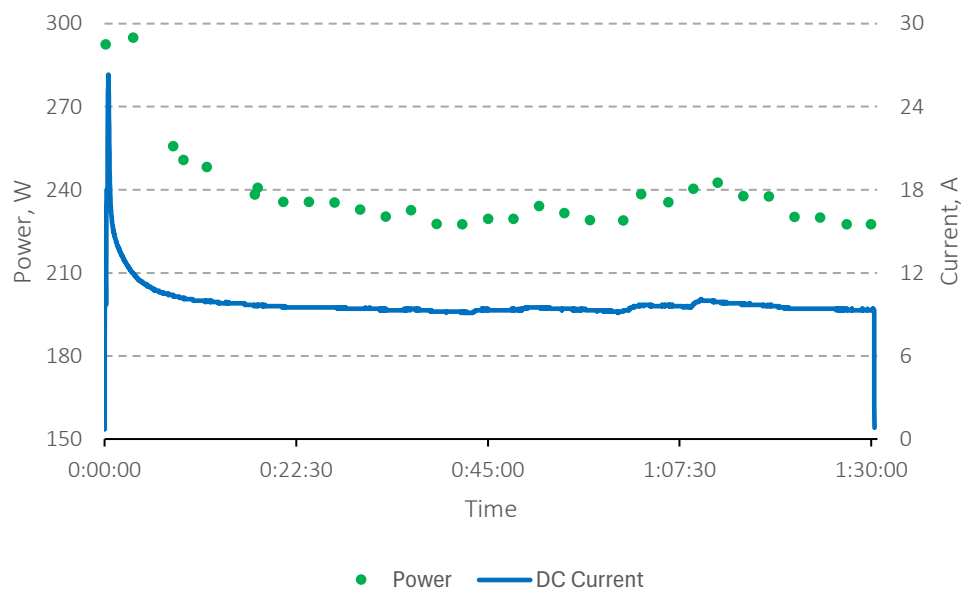
Figure 33: Beans cooking test with PTC-only cooker
