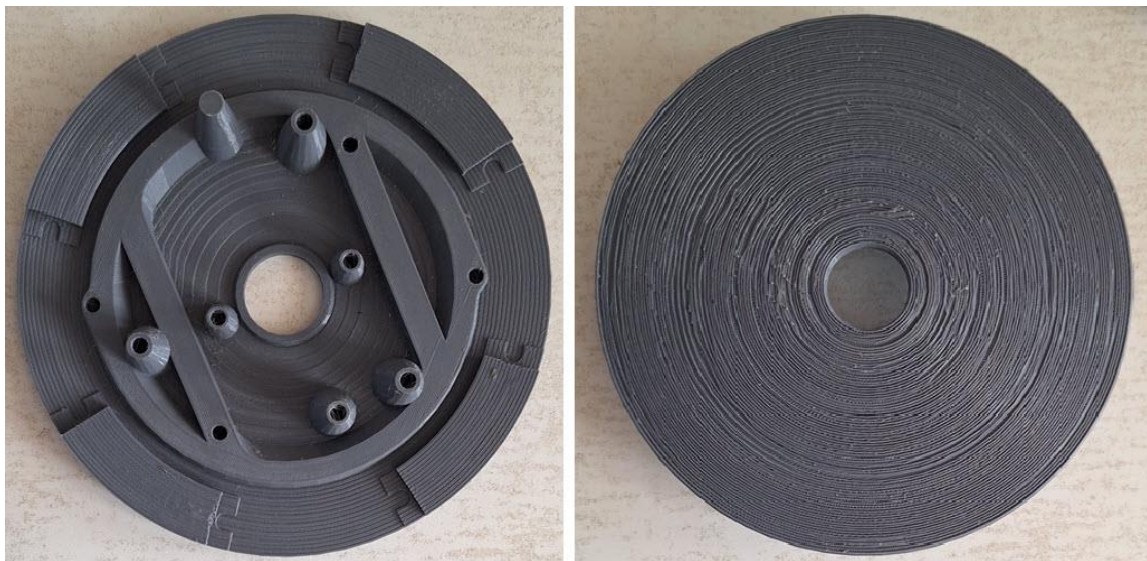
Figure 6: Initial 3D printed model of hybrid hot plate. Bottom view (left) and top view (right).
