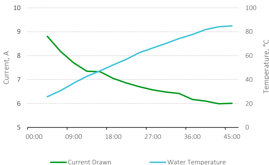
Figure 28: Water boiling test results conducted using the PTC-only EPC during the initial prototype tests
