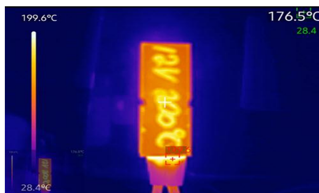
Figure 1: Lab test of a 12V 200°C PTC thermal distribution
