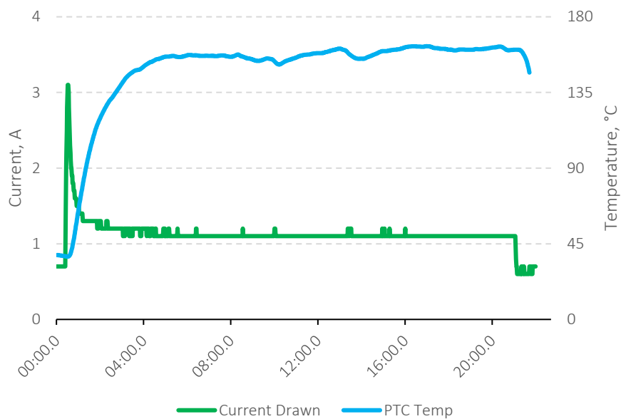
Figure 2: Current drawn and PTC temperature against time for a single PTC rated at 24V 200°C
