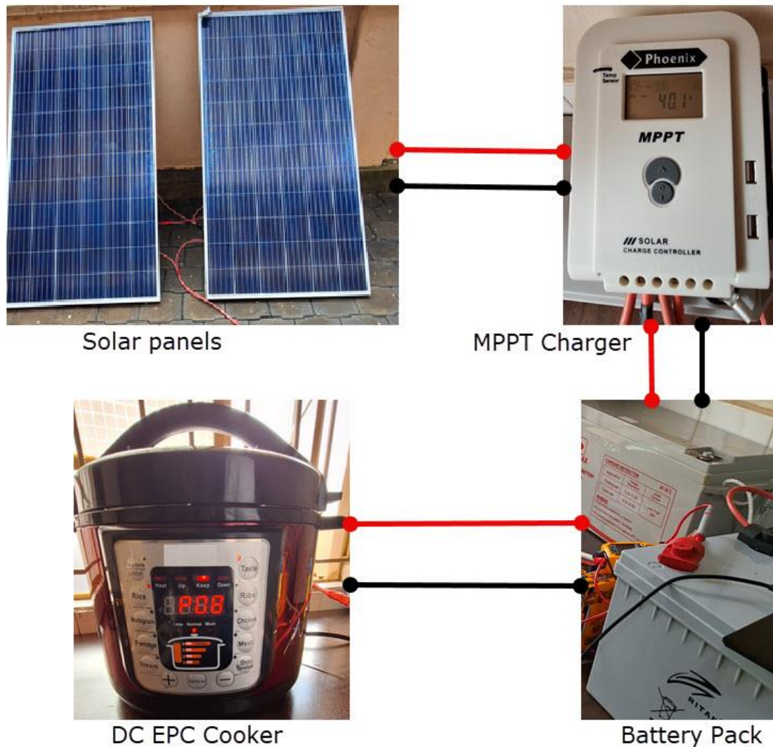
Figure 21: Solar PV system configuration
