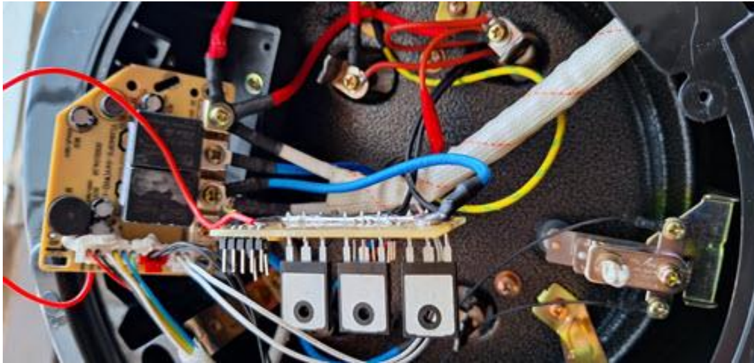
Figure 15: Hybrid circuitry. Both the main and PTC circuits are wired and connected and fitted in the DC pressure cooker
