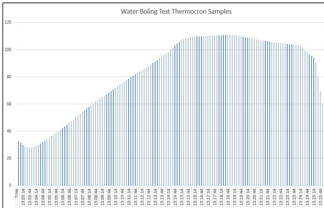
Figure 26: Graph water boiling samples. Temperature vs Time taken
