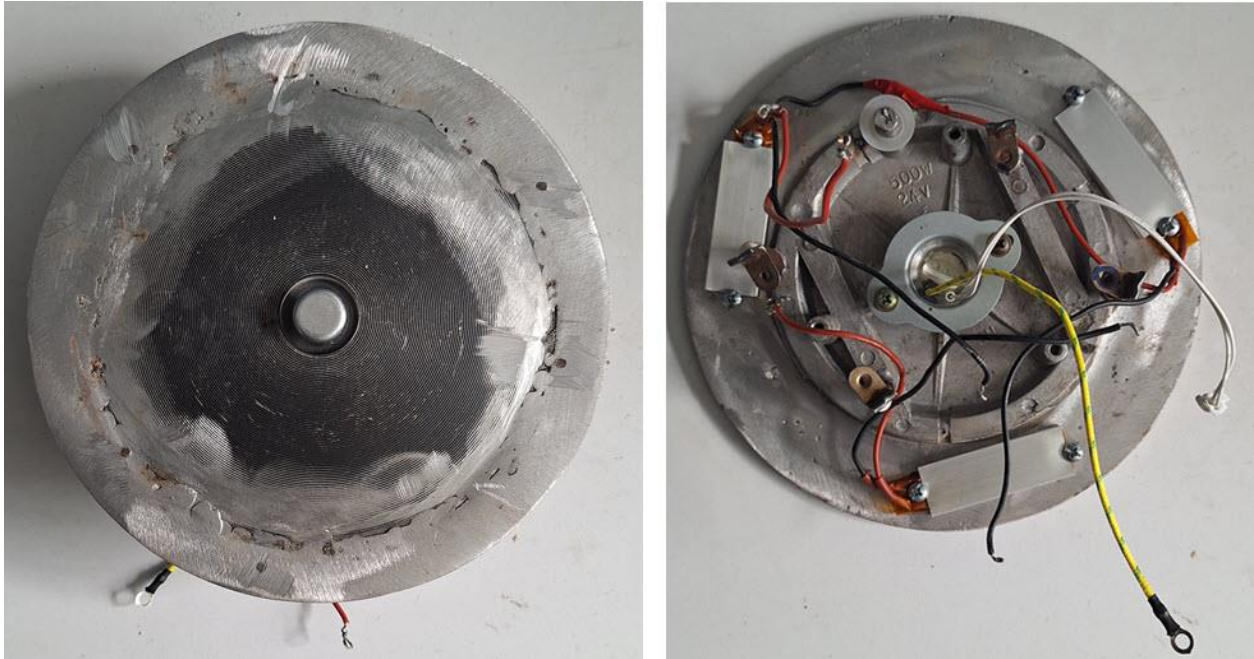
Figure 10: Hybrid hot plate casting with PTCs fixed.
