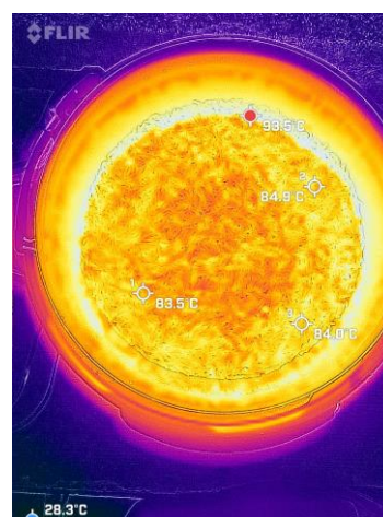
Figure 36: Final rice temperature for the hybrid EPC test
