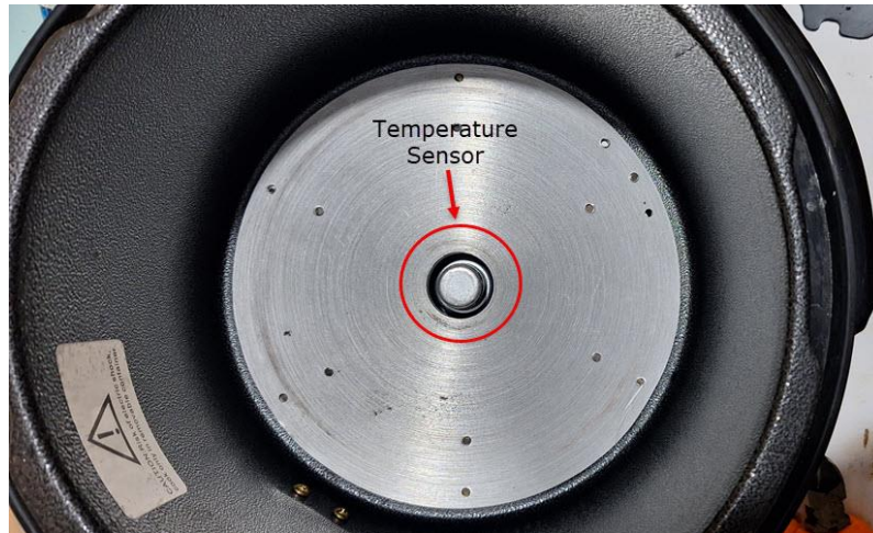
Figure 22: Location of cooking pot presence and temperature sensor
