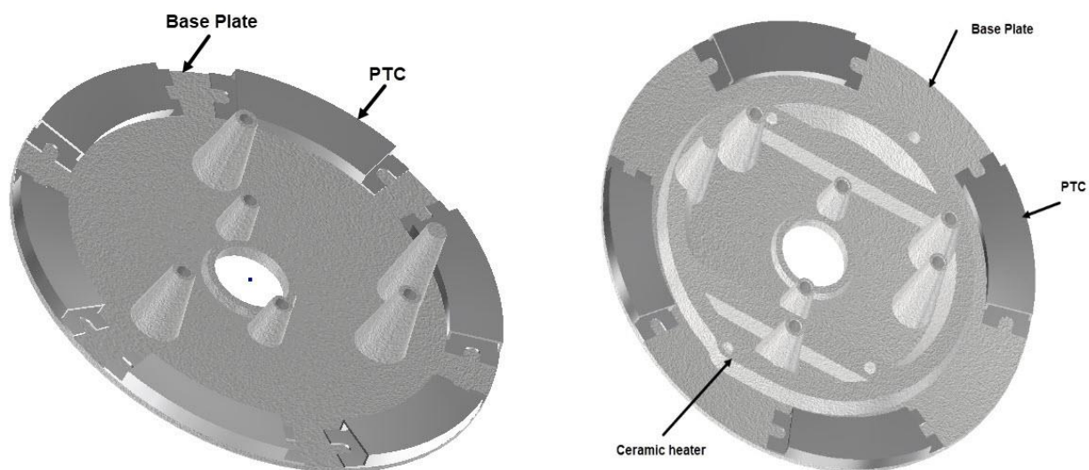
Figure 5: 3D CAD models of Hybrid and PTC only designs
