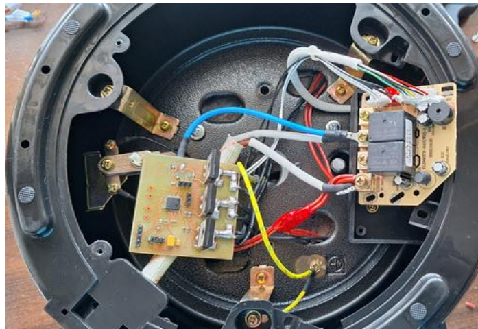
Figure 18: PTCs only circuitry. Both the main and PTC circuits are wired and connected and fitted in the DC pressure cooker
