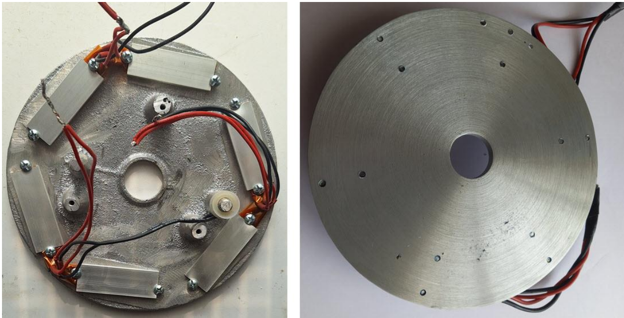
Figure 12: PTC only hot plate machined and fitted with PTCs heaters
