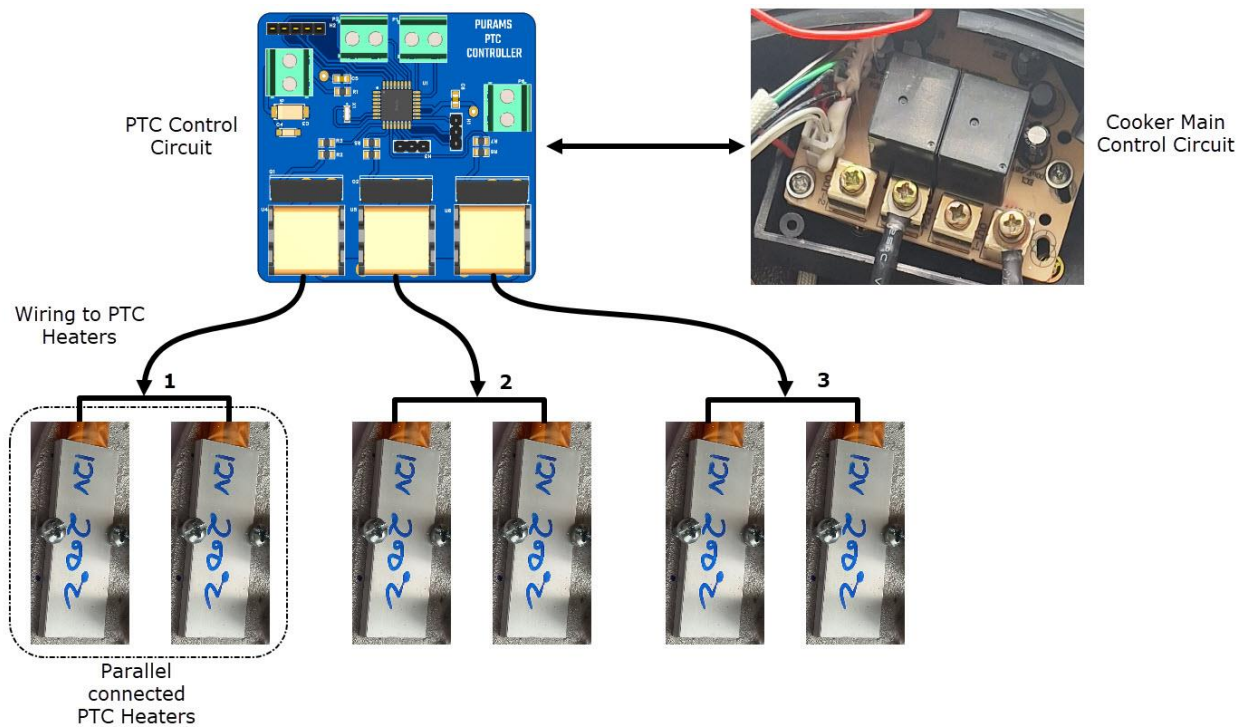
Figure 16: 2 PTCs are paired and the 3 pairs connected to the control board.
