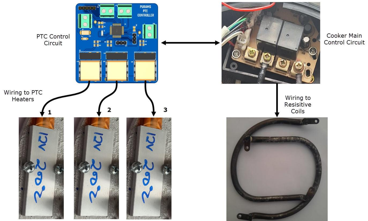
Figure 13: Wiring of the hybrid EPC heating elements (Resistive and PTC heaters)
