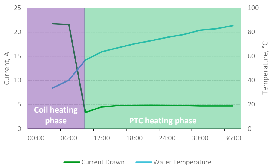
Figure 27: Water boiling test results conducted using the hybrid EPC during the initial prototype tests
