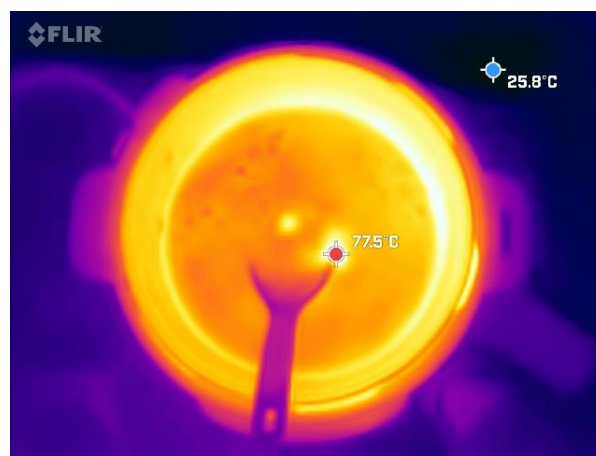
Figure 34: Final beans temperature for the PTC-only EPC test
